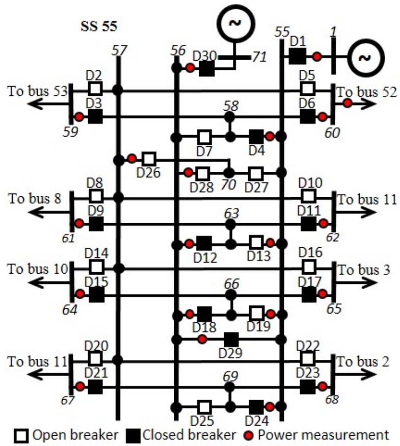
Figure 1: Substation diagram - 55-bus test system
