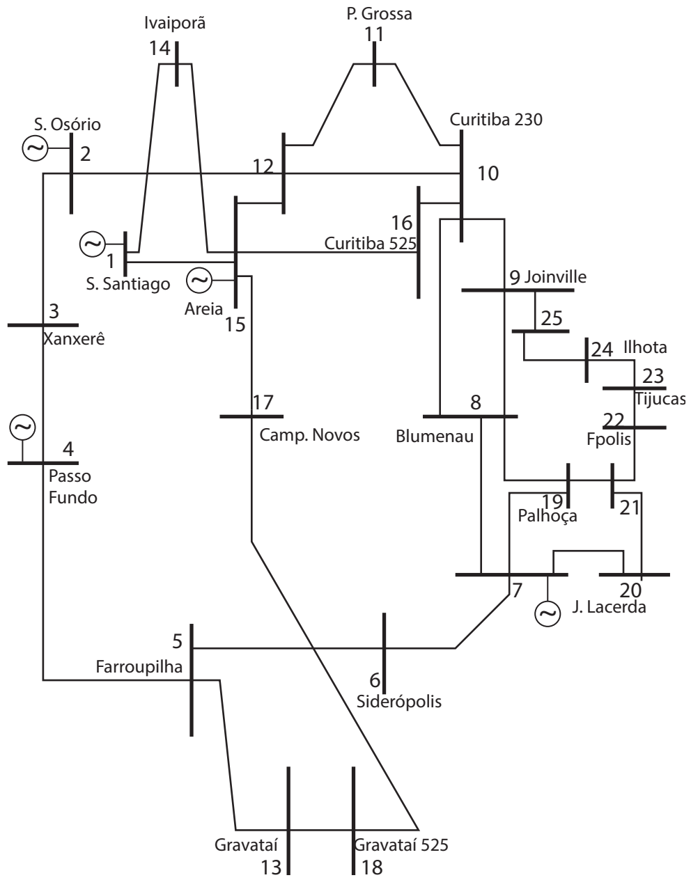
Figura 1: Diagram - 25-bus test system
